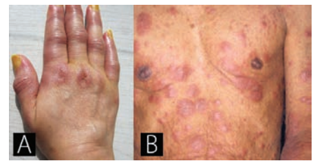
Gambar 2. Reaksi tipe 1/ reaksi reversa 9
